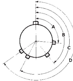
Viewed from front of plug
