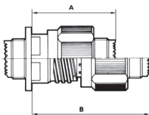
Type 0 with plug
