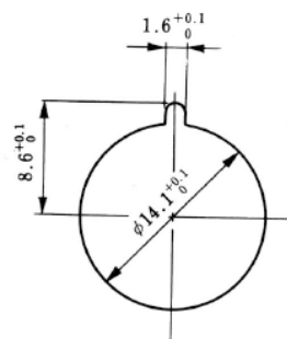
Type HR10A-13TR (Panel thickness 1 to 1.5mm)
