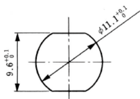
Type HR10A-10TR (Panel thickness 1 to 2mm)
