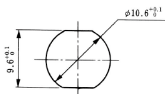
Type HR10A-10WTR (Panel thickness 1 to 2mm)
