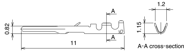
Male contact
