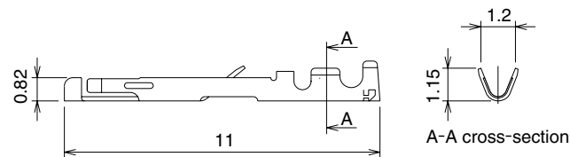
Female contact
