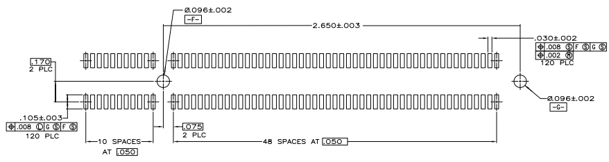
RECOMMENDED PC BOARD PATTERN (CONNECTOR SIDE SHOWN)
