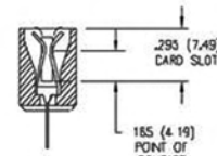
SECTION THROUGH CONTACT POSITION
