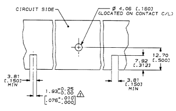
RECOMMENDED LAYOUT FOR P.C. BOARD SCALE 2:1
