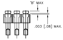
SAME AS FIG. 5 EXCEPT AS SHOWN (USED IN CSS CABLE) FIGURE 6 (SEE NOTE 9 SHT.1)
