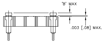
FIGURE 8 OPTION -N (SEE NOTE 9 SHT.1) "B" DIMENSION FOR OPTION -N = NON FLUSH
