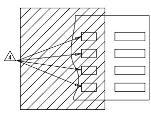
RECOMMENDED PCB LAYOUT FOR 1954289-2 & 1-1954289-2
