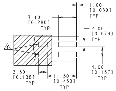
RECOMMENDED PCB LAYOUT FOR 1954289-1 & 1-1954289-1
