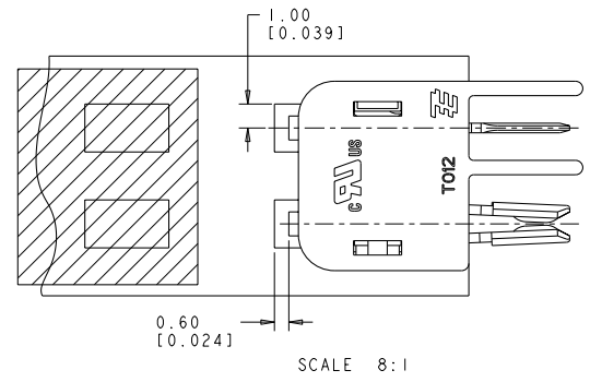
RECOMMENDED PCB LAYOUT FOR 1954289-1 & 1-1954289-1
