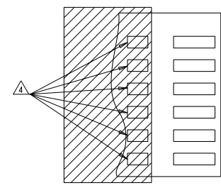
RECOMMENDED PCB LAYOUT FOR 1954289-3 & 1-1954289-3
