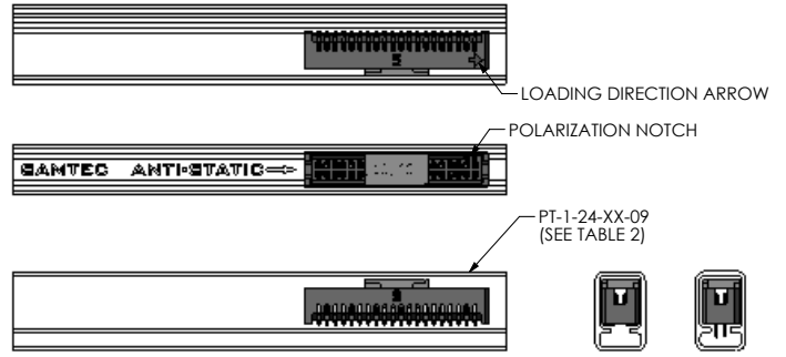
FIGURE 4 -TR: TAPE AND REEL
