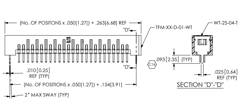
FIGURE 6 -WT OPTION (DIFFERENT AS SHOWN, OTHERWISE SAME AS FIG. 1)
