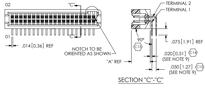
FIGURE 5 -RA OPTION (DIFFERENT AS SHOWN, OTHERWISE SAME AS FIG. 1)
