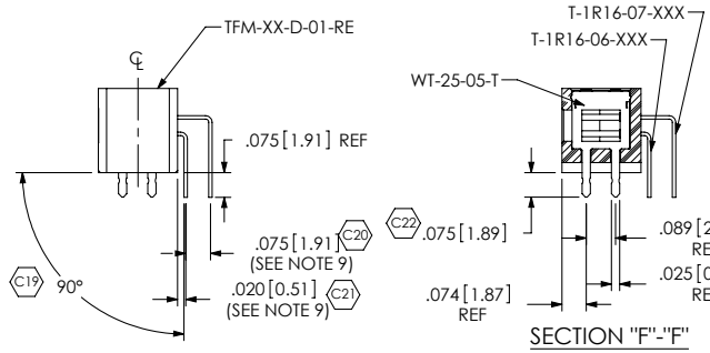
FIGURE 12 -RE2: RIGHT ANGLE ELEVATED .093 PCB DIFFERENT AS SHOWN, OTHERWISE SAME AS FIG. 1 NOT RELEASED FOR PRODUCTION
