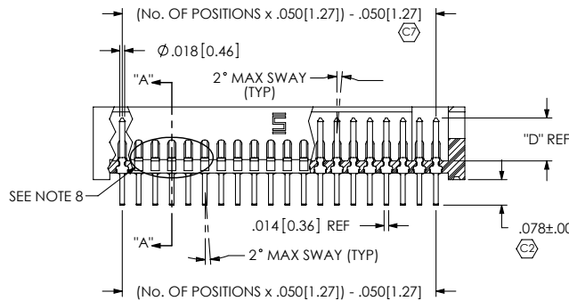
FIGURE 1 THROUGH HOLE -01, -11, -21, -31
