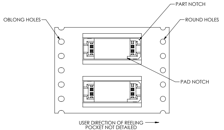
FIGURE 4 -TR: TAPE AND REEL
