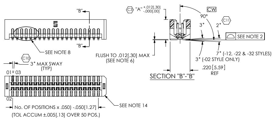
FIGURE 2 THROUGH HOLE -02, -12, -22, -32 (DIFFERENT AS SHOWN, OTHERWISE SAME AS FIG. 1)
