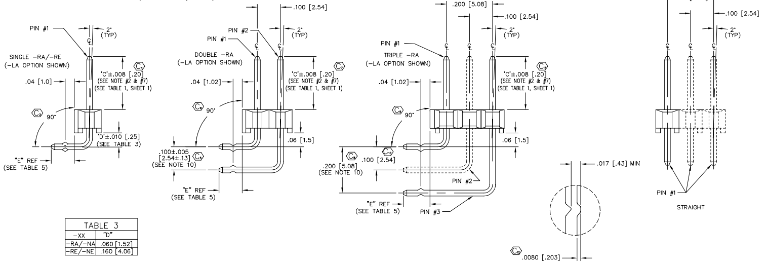
CRIMP DETAIL SCALE: 2x [TYP- ALL CRIMPS]
