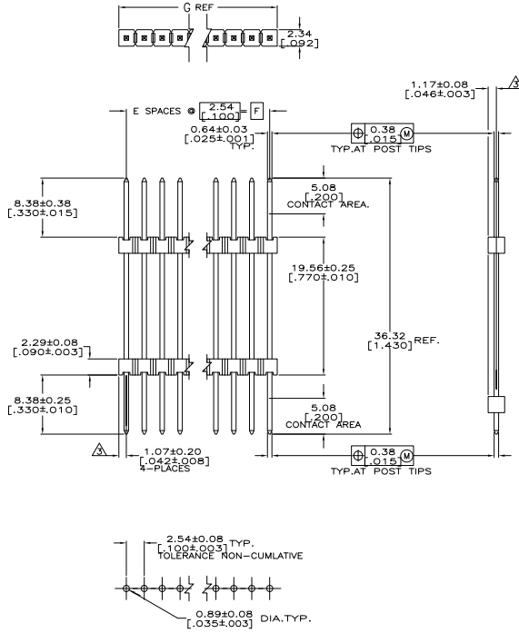
RECOMMENDED HOLE LAYOUT
