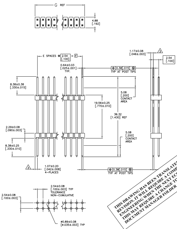
RECOMMENDED HOLE LAYOUT
