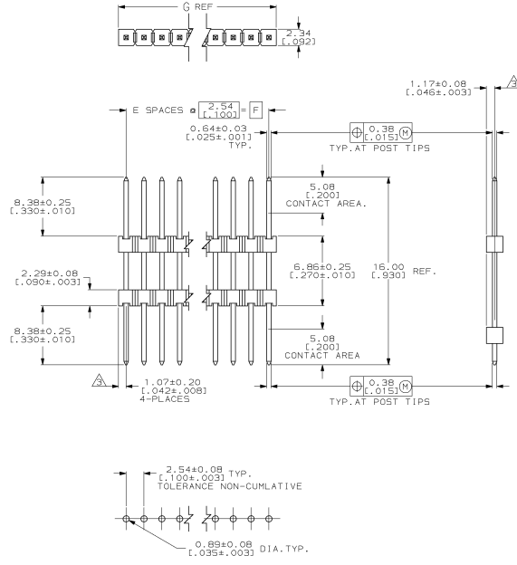
RECOMMENDED HOLE LAYOUT
