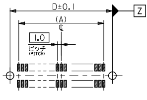
推奨基板寸法 (34, 50, 66極) RECOMMENDED PCB PATTERN LAYOUT (34,50,66 CKTS.) (SCALE 2-1)
