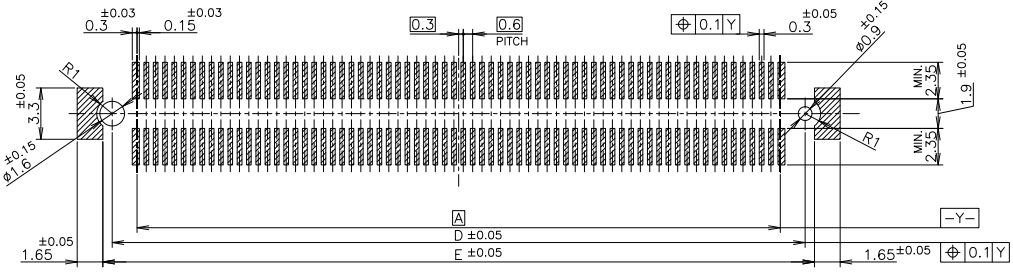
REFERENCE P.C. BOARD LAYOUT
