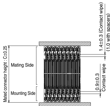
Mating Cross Section(FREE) Mating condition without spacers
