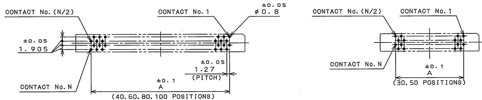
APPLICABLE P.C.B. DIMENSION(REF.)
