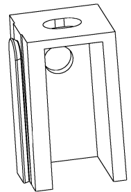
1445729-1 WITHOUT LOCKING FEATURE, OVAL MOUNTING HOLE
