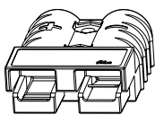
647845-4 AND 647845-7 SCALE 2:1
