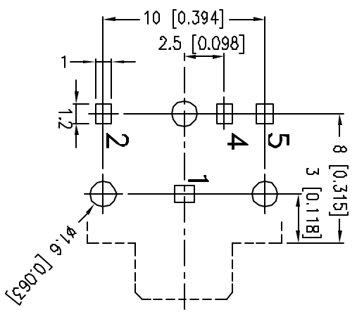
HOLE LAYOUT (TOP VIEW)
