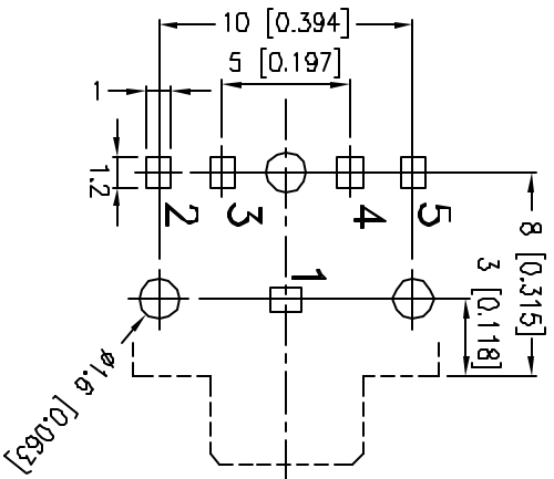
HOLE LAYOUT (TOP VIEW)
