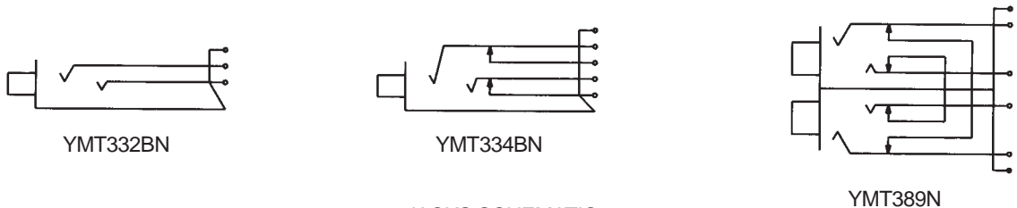
JACKS SCHEMATIC "N" SUFFIX DENOTES WELDED GOLD CONTACTS AND NICKEL-PLATED FRAME
