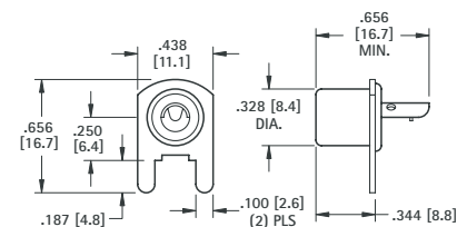
Mounting Detail
