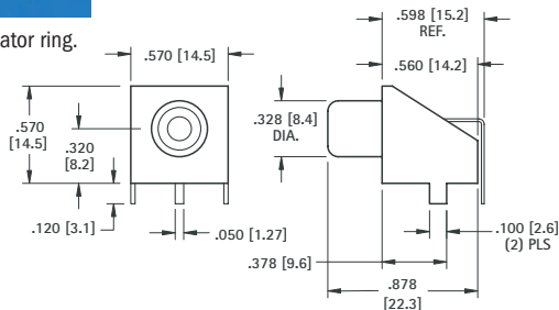
Mounting Detail
