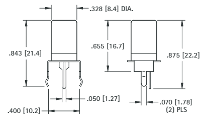
Mounting Detail
