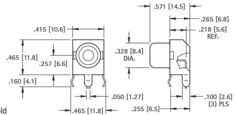
Mounting Detail
