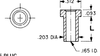
ACCEPTS .175 PLUG
