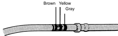
Socket M39029/12-148
