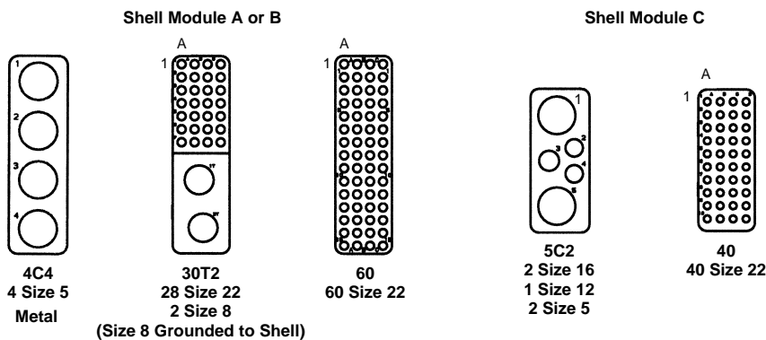
Shell Size 1 Plug Rear Release/Remove Contacts
