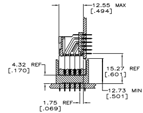
REFERENCE MATED CROSS SECTION SCALE 2:1
