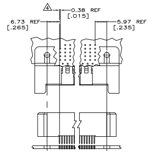
REFERENCE MATED CONNECTOR THRU HOLE OFFSET SCALE 2:1
