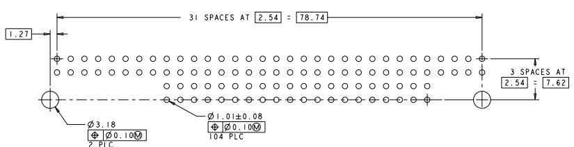
RECOMMENDED PCB LAYOUT FOR 1375961-2 & -4
