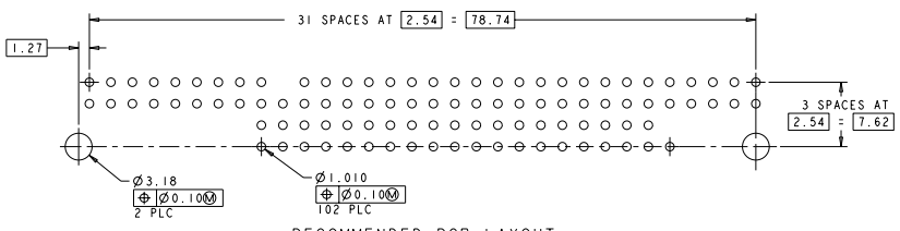
RECOMMENDED PCB LAYOUT FOR 1375961-1 & -3
