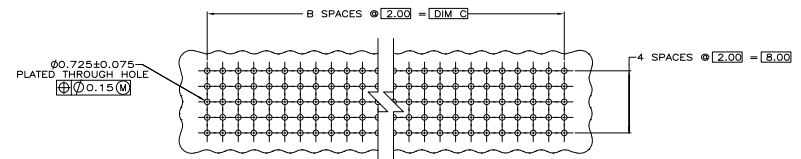
RECOMMENDED CIRCUIT PATTERN (COMPONENT SIDE)
