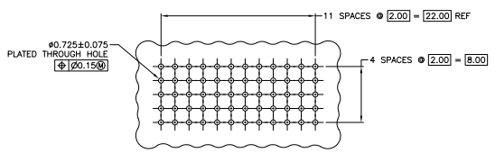
RECOMMENDED CIRCUIT PATTERN (COMPONENT SIDE)
