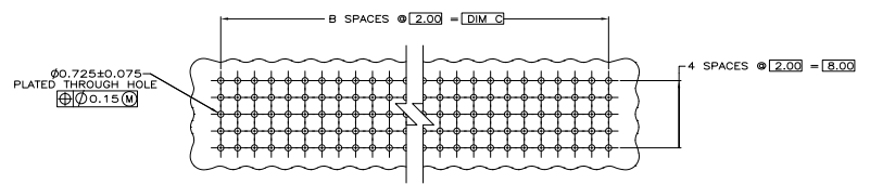
RECOMMENDED CIRCUIT PATTERN (COMPONENT SIDE)
