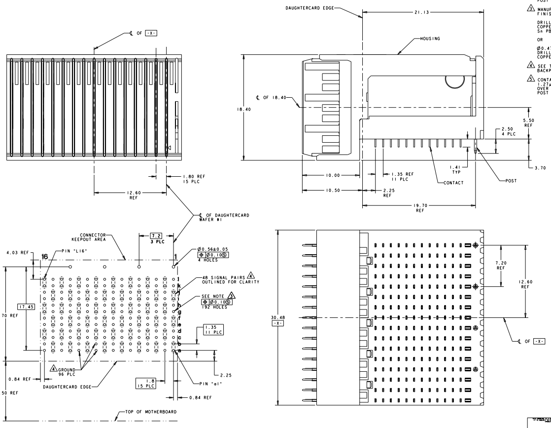
PC BOARD LAYOUT (CONNECTOR SIDE) SCALE: 5:1
