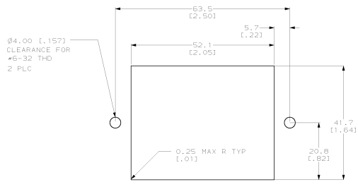
RECOMMENDED STATIONARY MOUNT PANEL CUTOUT EXTERNAL VIEW
