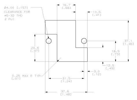
RECOMMENDED STATIONARY MOUNT PANEL CUTOUT EXTERNAL VIEW
