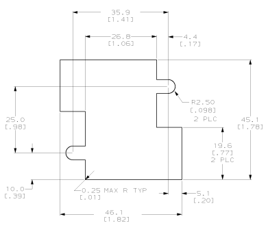
RECOMMENDED FLOAT MOUNT PANEL CUTOUT EXTERNAL VIEW
