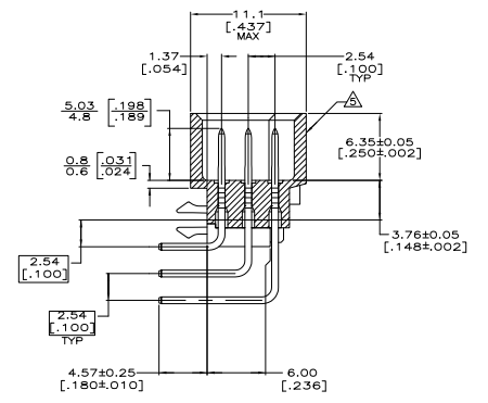
SECTION Z-Z
