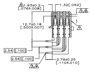
SECTION Y-Y
