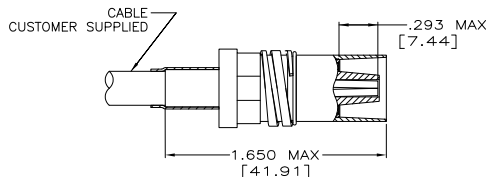
ASSEMBLED VIEW SCALE 2:1
