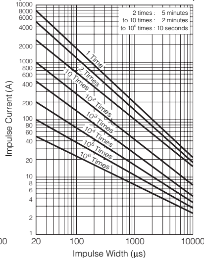
20 Series (ERZC20EK361 to ERZC20EK681)
