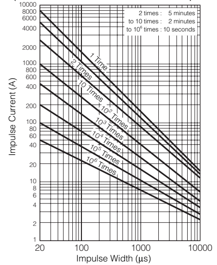
20 Series (ERZC20EK751 to ERZC20EK112)
