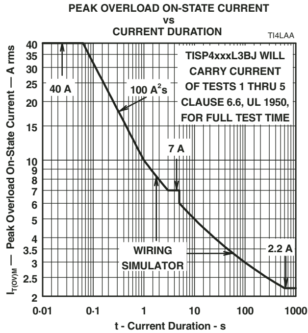
Figure 2. Peak Overload On-state Current against Duration
