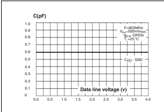
Figure 1. Line capacitance versus line voltage (typical values)
