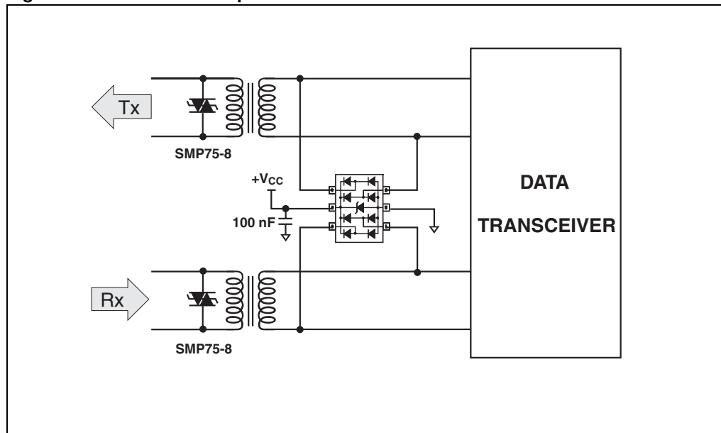
Figure 6. T1/E1/Ethernet protection
