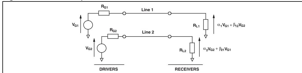
Figure 14. Crosstalk phenomena
