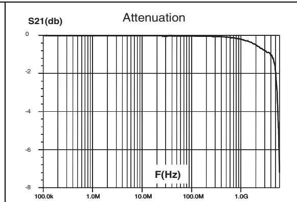
Figure 4. Frequency response
