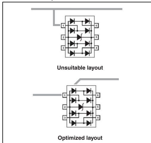
Figure 10. ESD behavior: layout optimization
