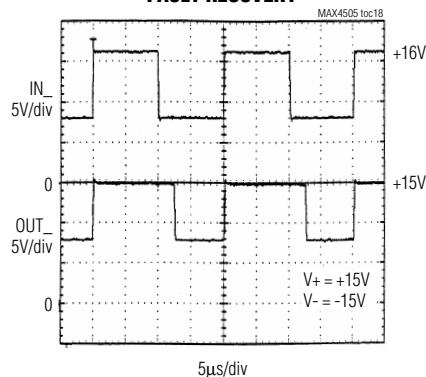
FAULT RECOVERY
