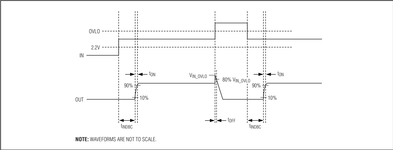
Figure 1. Timing Characteristics
