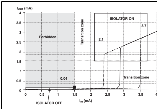
Figure 7. Current transfer characteristic
