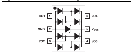
Figure 1. Functional diagram
