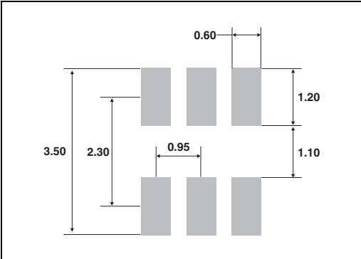
Figure 20. SOT23-6L footprint (mm)
