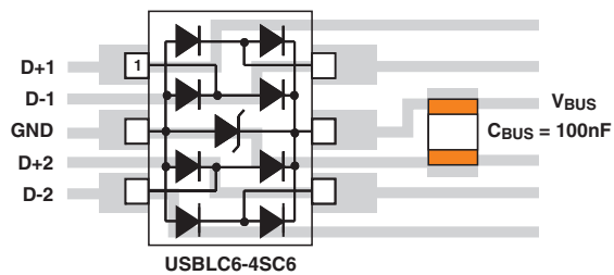
Figure 18. USBLC6-4SC6 PCB layout considerations
