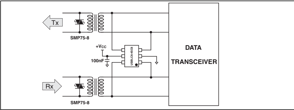
Figure 15. T1/E1/Ethernet protection
