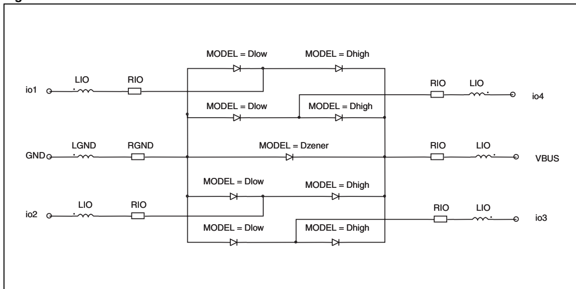
Figure 16. PSPICE model
