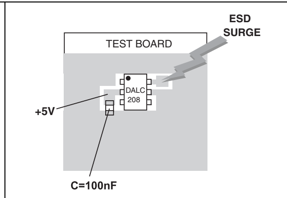
Figure 10. ESD behavior: measurement conditions (with coupling capacitance)
