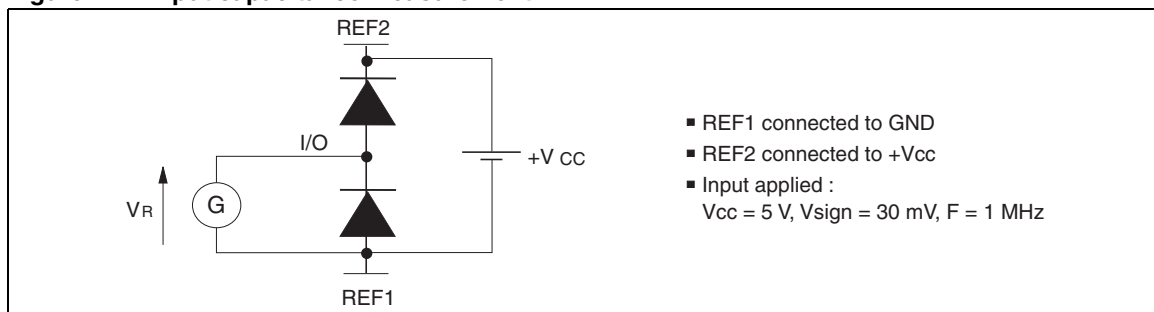
Figure 2. Input capacitance measurement
