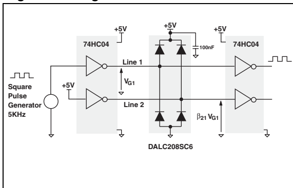
Figure 14. Digital crosstalk measurements
