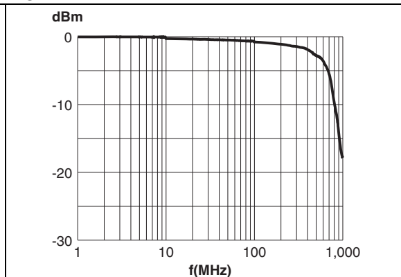
Figure 18. DALC208SC6 attenuation
