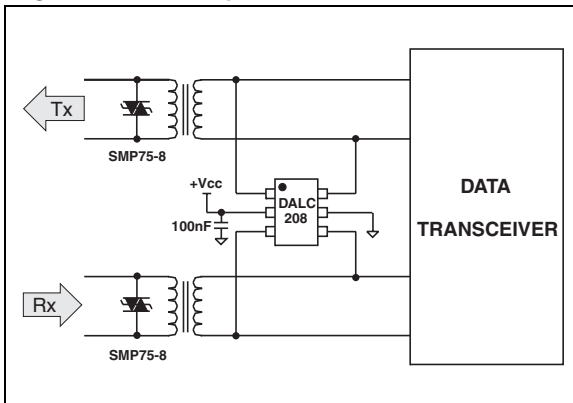
Figure 22. Another way to connect the DALC208SC6
