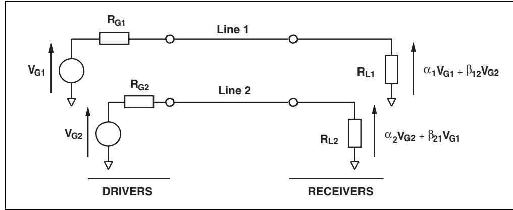
Figure 13. Crosstalk phenomena
