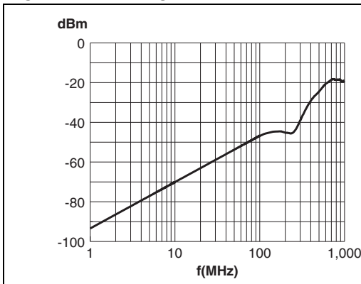
Figure 17. Analog crosstalk results
