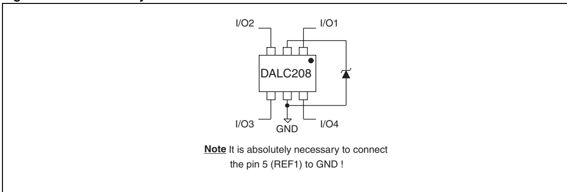
Figure 22. Another way to connect the DALC208SC6
