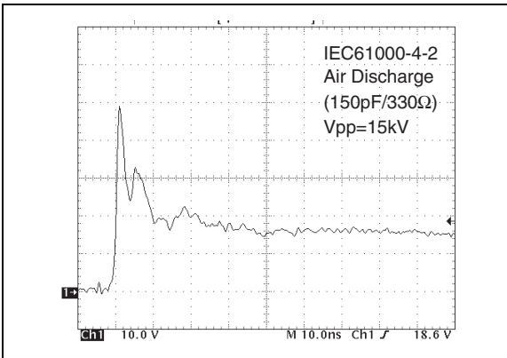
Figure 11. Remaining voltage after the DALC208SC6 during positive ESD surge
