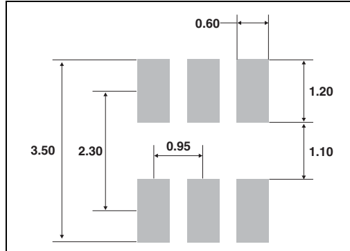
Figure 22. SOT23-6L footprint
