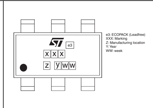
Figure 23. SOT23-6L marking
