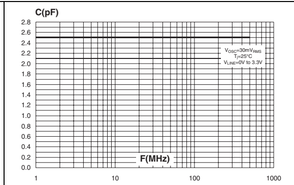
Figure 5. Frequency response
