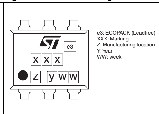
Figure 21. SOT-666 marking
