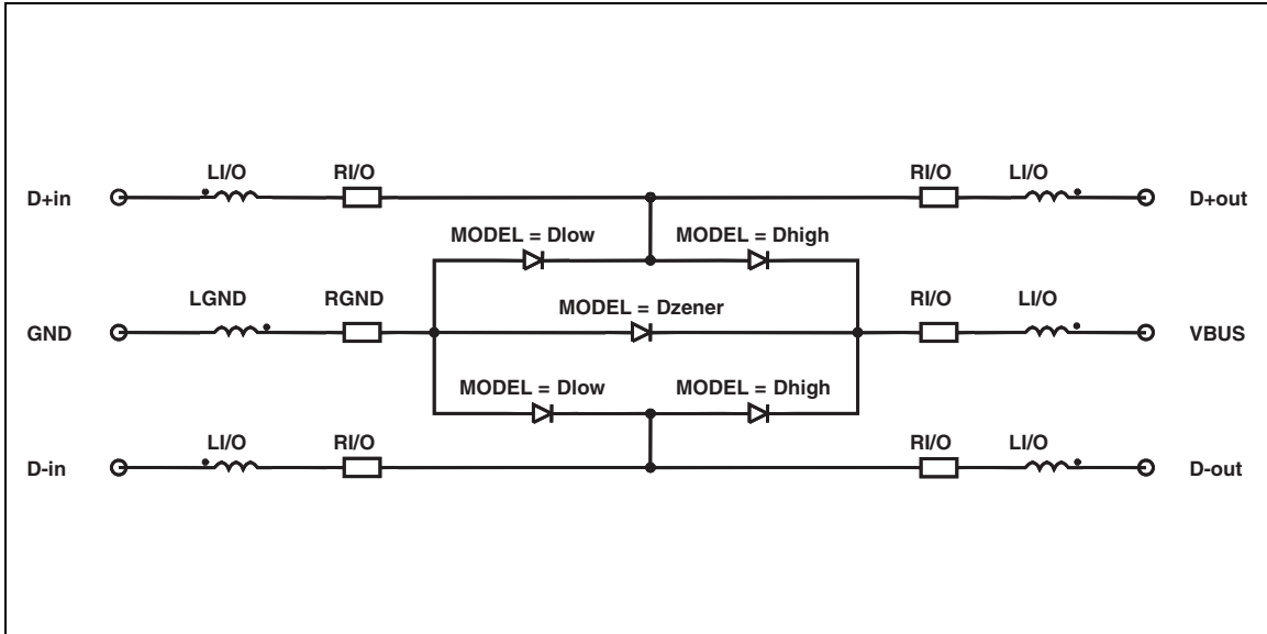
Figure 16. PSpice model
