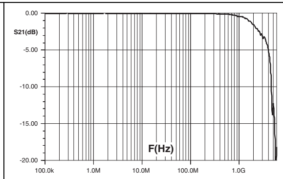
Figure 5. Frequency response
