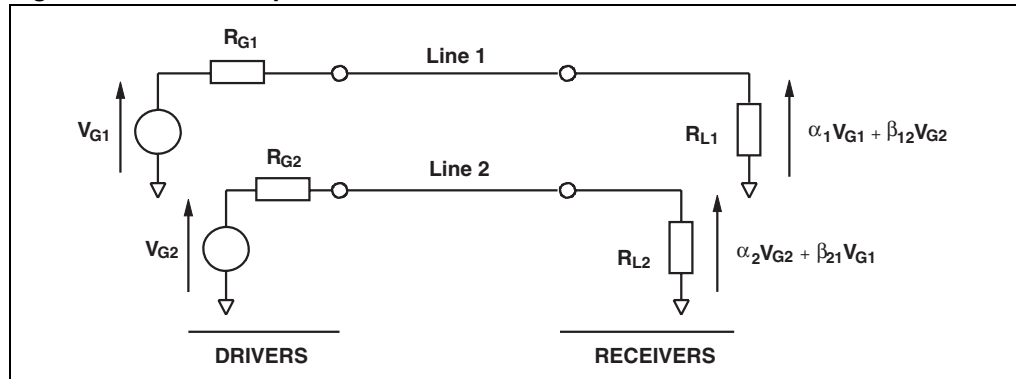
Figure 11. Crosstalk phenomenon
