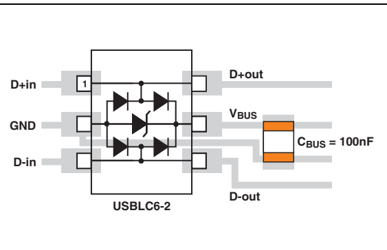
Figure 18. USBLC6-2 PCB layout considerations
