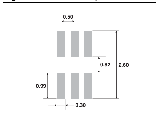
Figure 20. SOT-666 footprint
