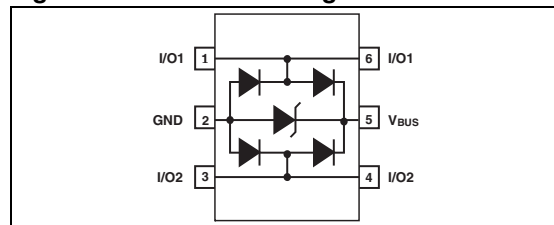
Figure 1. Functional diagram
