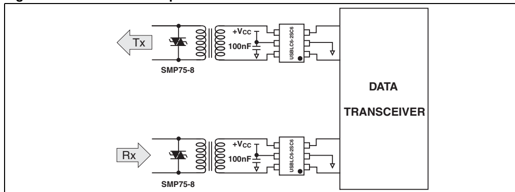
Figure 15. T1/E1/Ethernet protection
