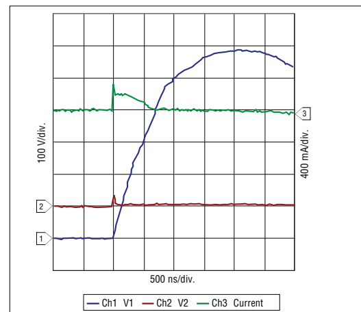
P850-G Solution: 4000 V Lightning 10/700 µsec, 100 A
