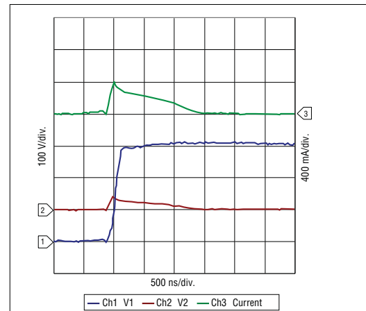
P500-G Solution: 5000 V Lightning 2/10 µsec, 500 A
