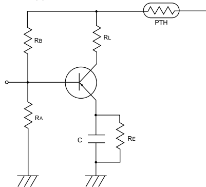
(1) Transistor Protection Circuit
