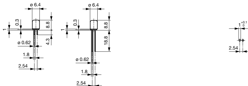
Drilling diagram
