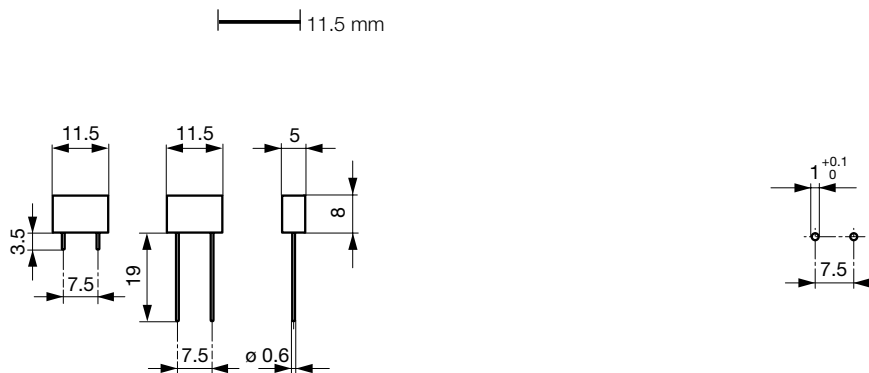
Drilling diagram
