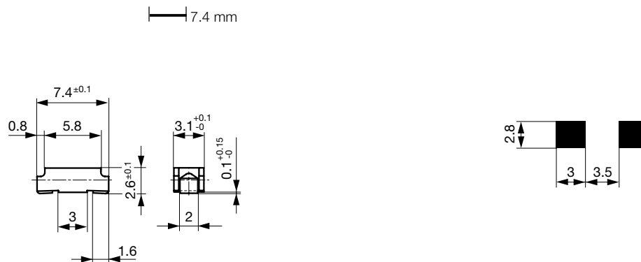
Soldering pads
